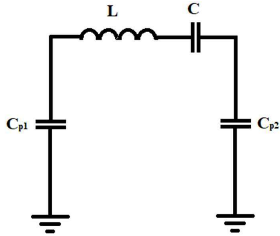
Fig.2 Equivalent circuit model of the interdigital-based structure
