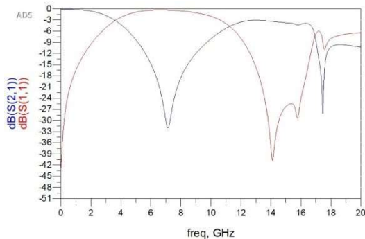
Fig. 4 S-parameter Characteristics performance of the proposed structure
