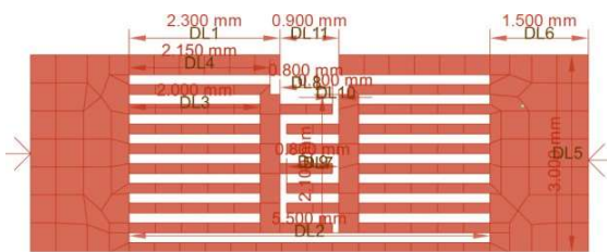
Fig.3 Dimensions of Filter
