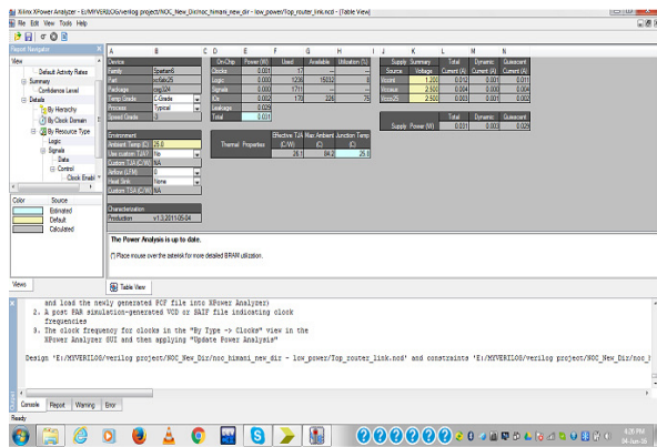
Fig. 12 Total Power Dissipation in ink Design II.
