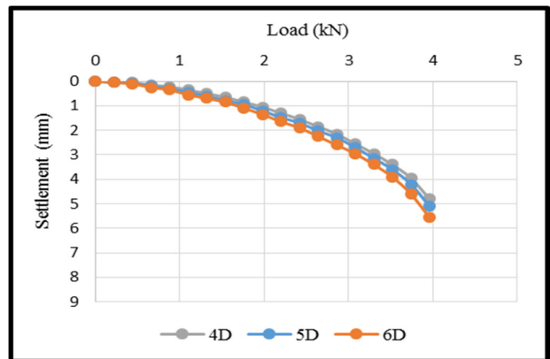
Fig -8: Load-Settlement curve based on pile spacing
