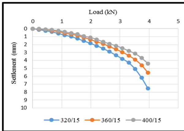
Fig -9: Load-Settlement curve based on pile depth
