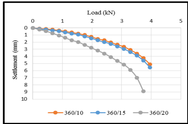
Fig -7: Load-Settlement curve based on cushion thickness
