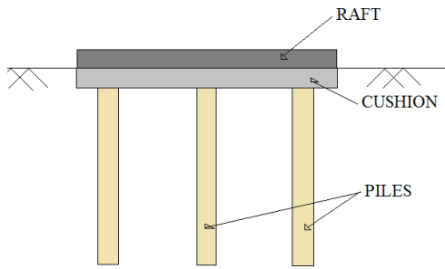
Fig -1: Disconnected piled raft foundation
