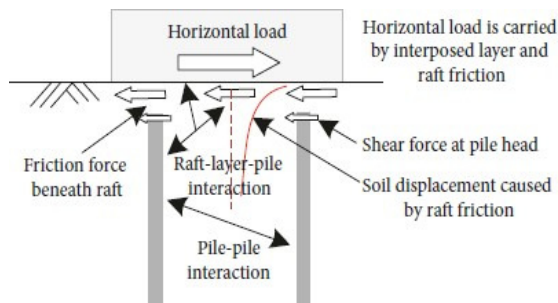
Fig -2: Horizontal load distribution technique
