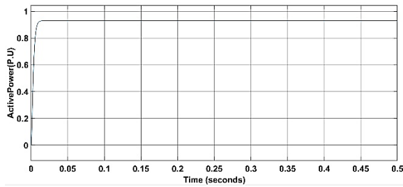
Figure 16: Active Power
