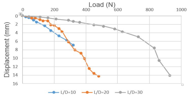
Fig.2 Variation of lateral load with pile displacement for pile group for all L/D ratios
