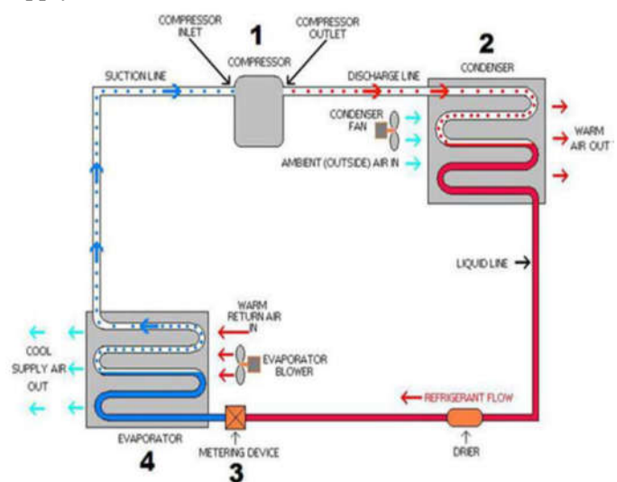
Fig -1: Refrigeration Cycle
